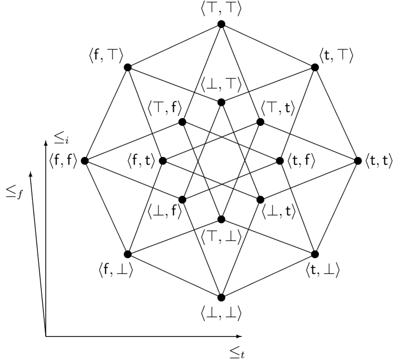
Figure 3: The trilattice SIXTEEN_3 represented as FOUR_2 \odot FOUR_2 .
