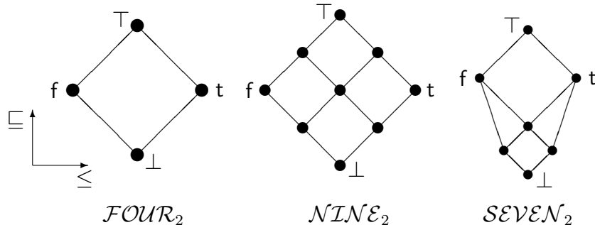
Figure 1: Some examples of (pre-)bilattices
